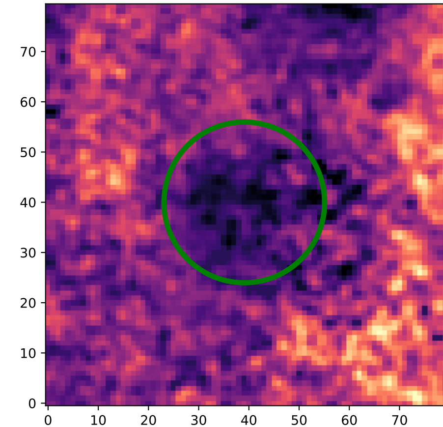
Region: 21 HI - Type 1
