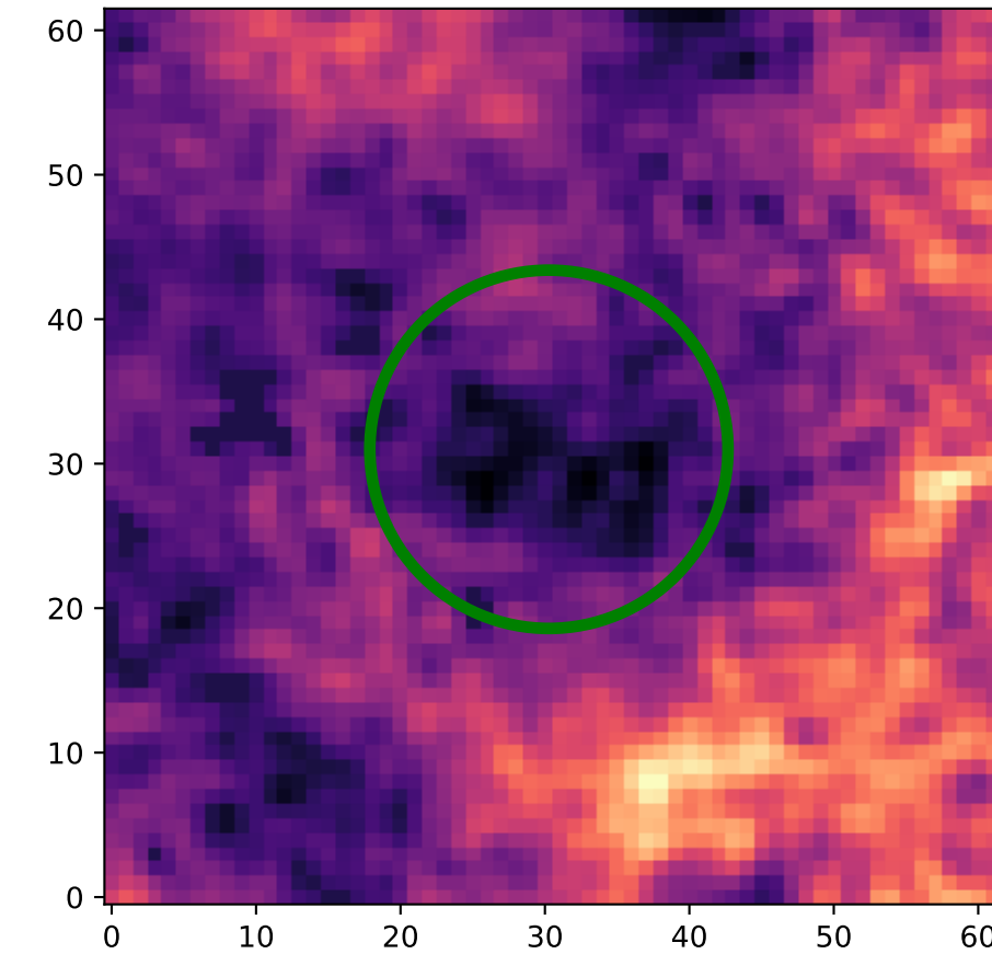
Region: 11 HI - Type 3
