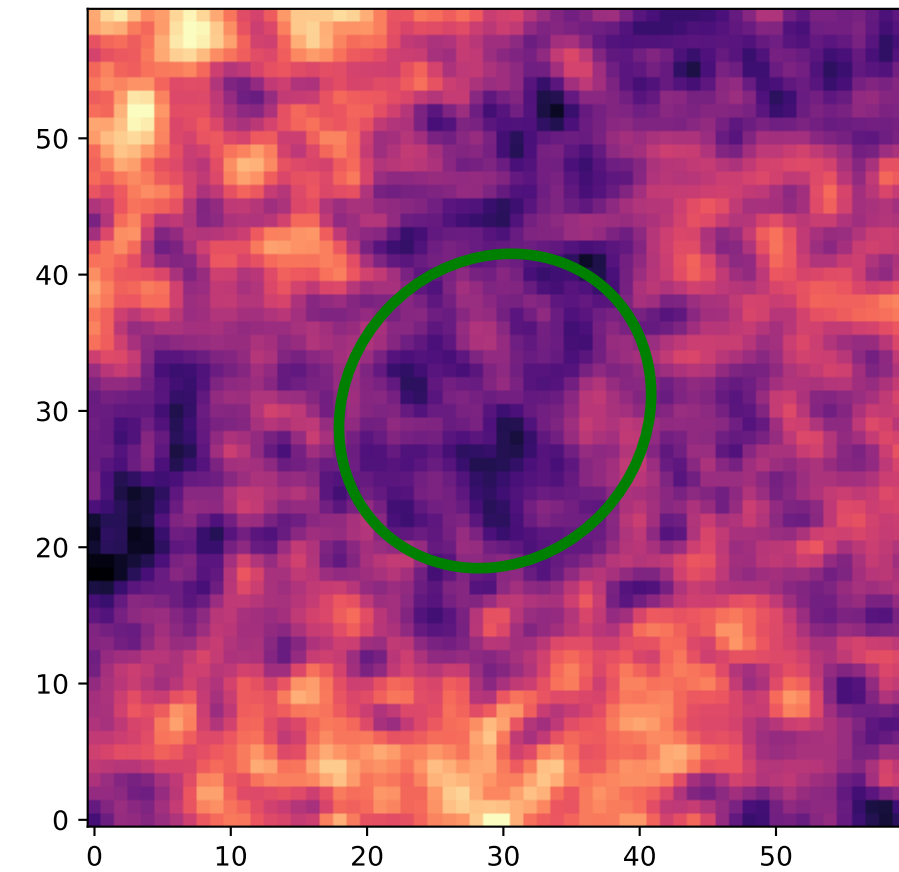
Region: 6 HI - Type 1
