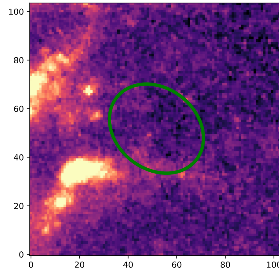
IRAC 8 micron - Classification: Diffuse
