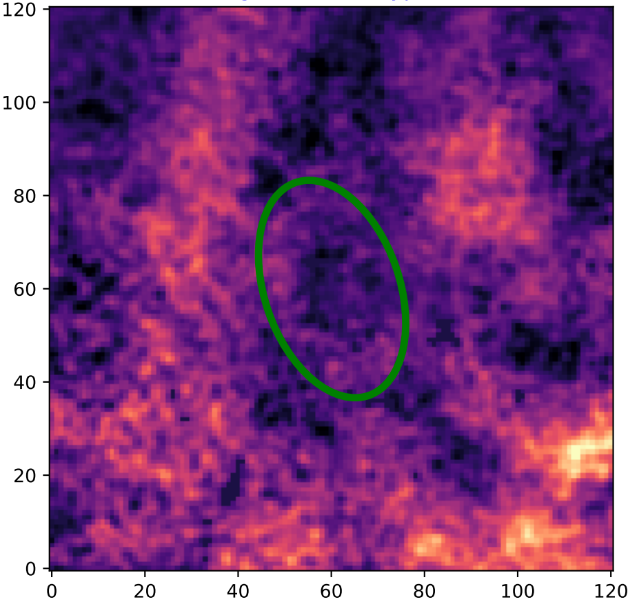
Region: 15 HI - Type 1
