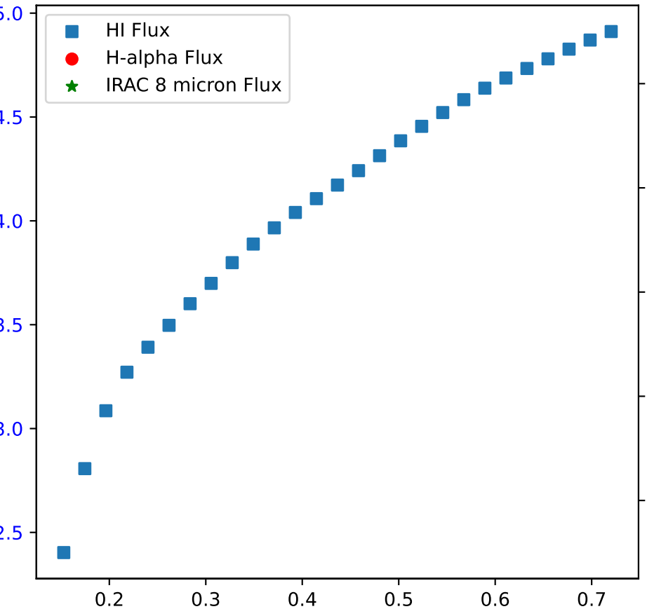
Flux of HI vs. H-alpha in Galaxy: NGC 4214 - Region 14
