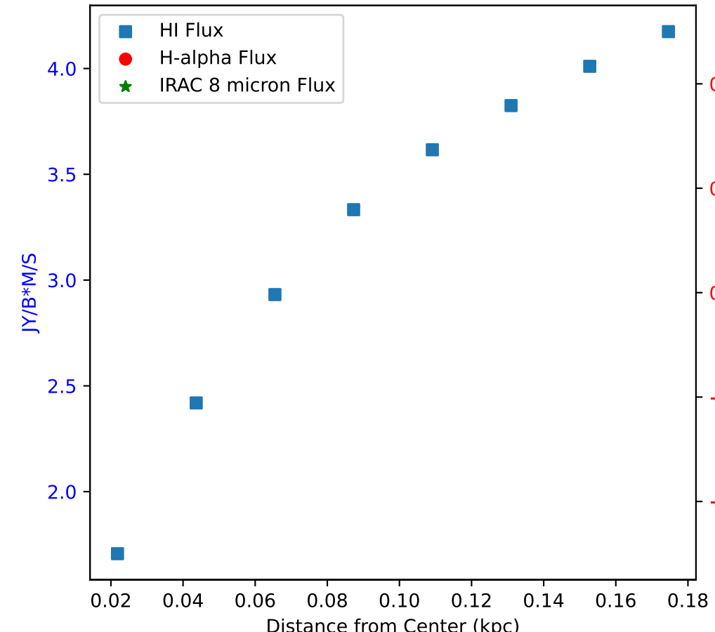
Flux of HI vs. H-alpha in Galaxy: NGC 4214 - Region 16
