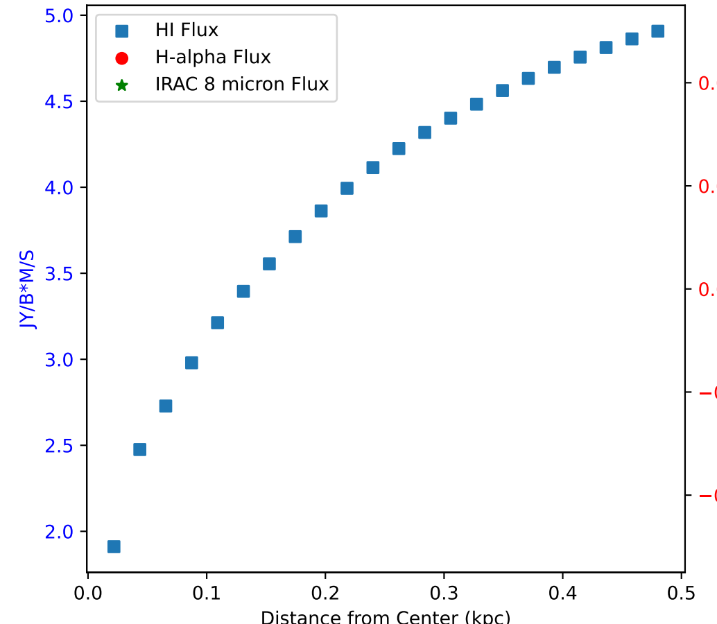
Flux of HI vs. H-alpha in Galaxy: NGC 4214 - Region 17
