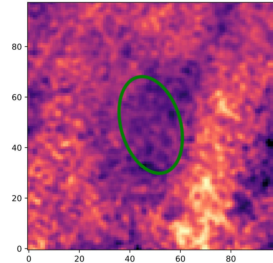
Region: 18 HI - Type 2
