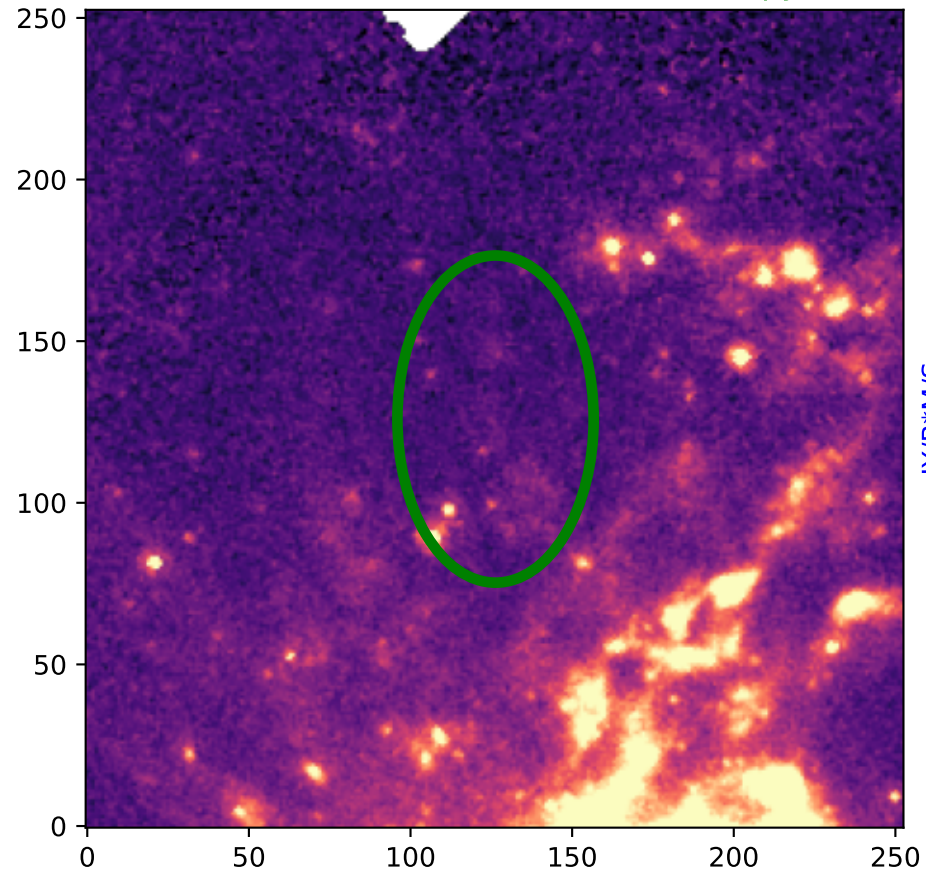
IRAC 8 micron - Classification: Clumpy
