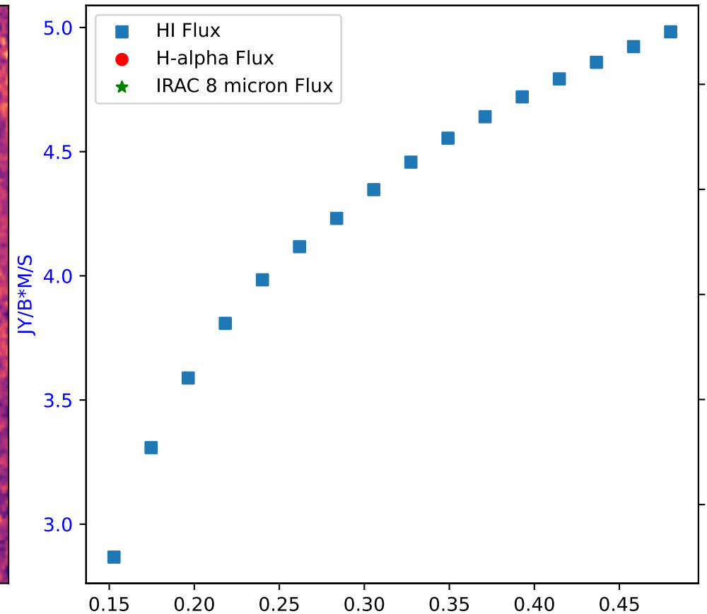
Flux of HI vs. H-alpha in Galaxy: NGC 4214 - Region 21
