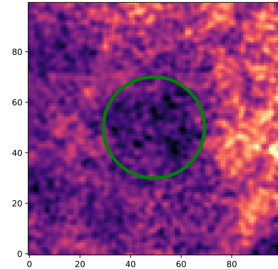
Region: 20 HI - Type 1
