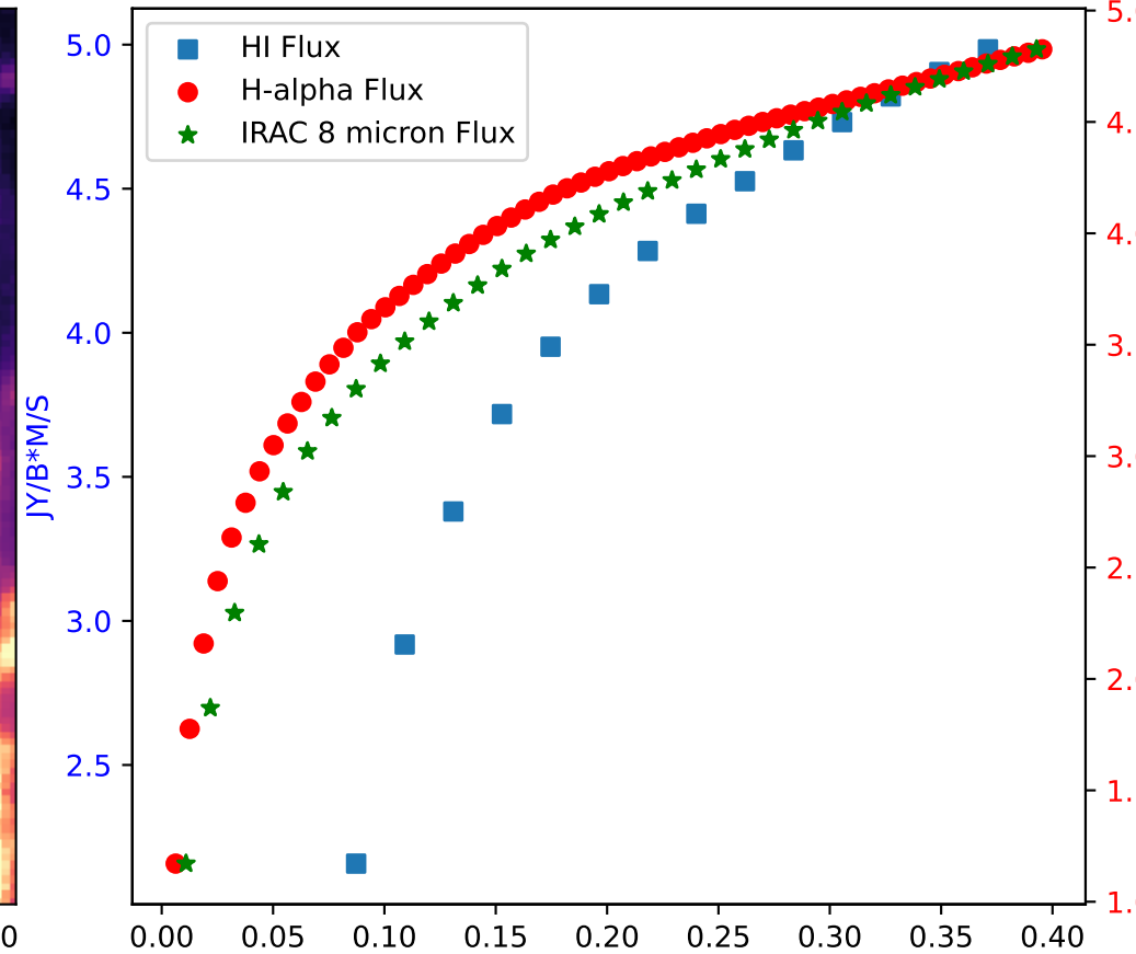
Flux of HI vs. H-alpha in Galaxy: NGC 4214 - Region 11
