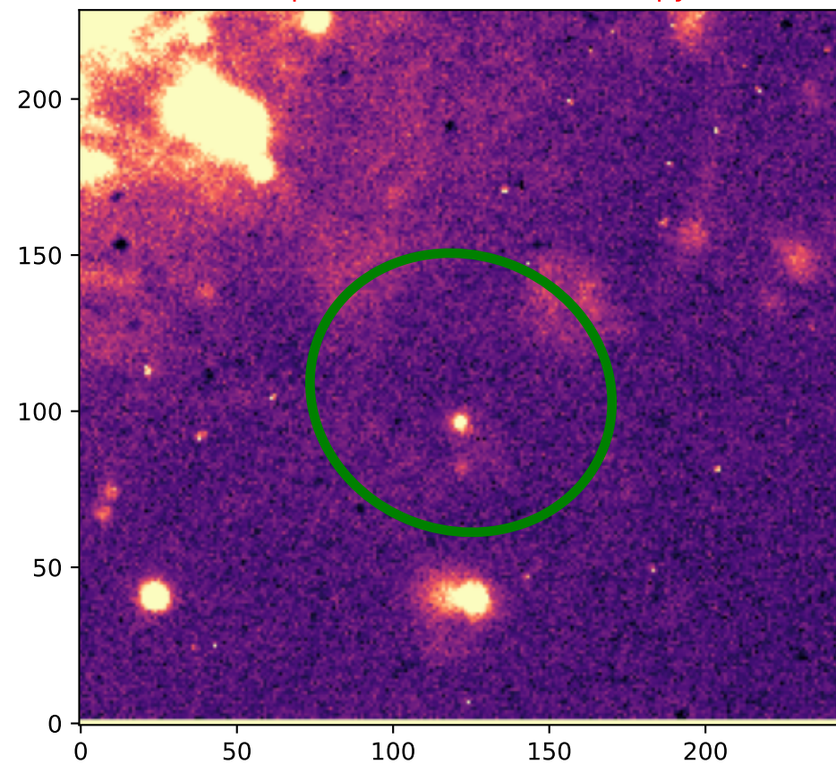
H-alpha - Classification: Clumpy
