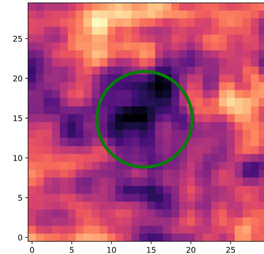
Region: 9 HI - Type 1
