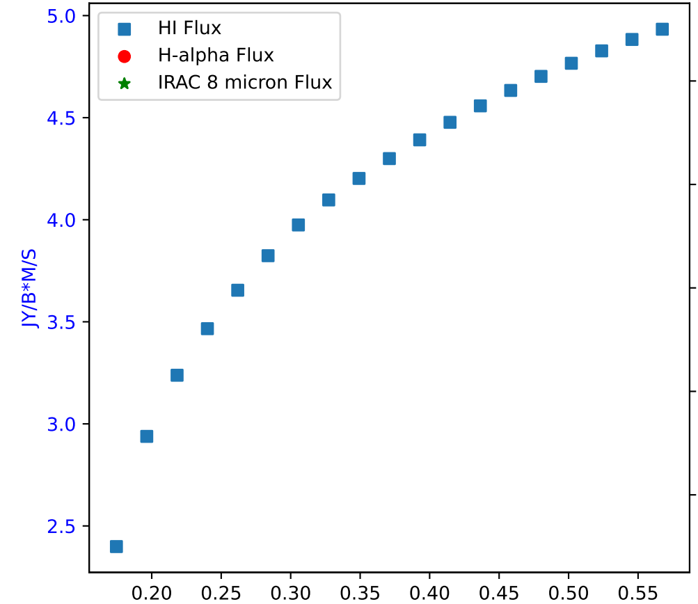
Flux of HI vs. H-alpha in Galaxy: NGC 4214 - Region 3
