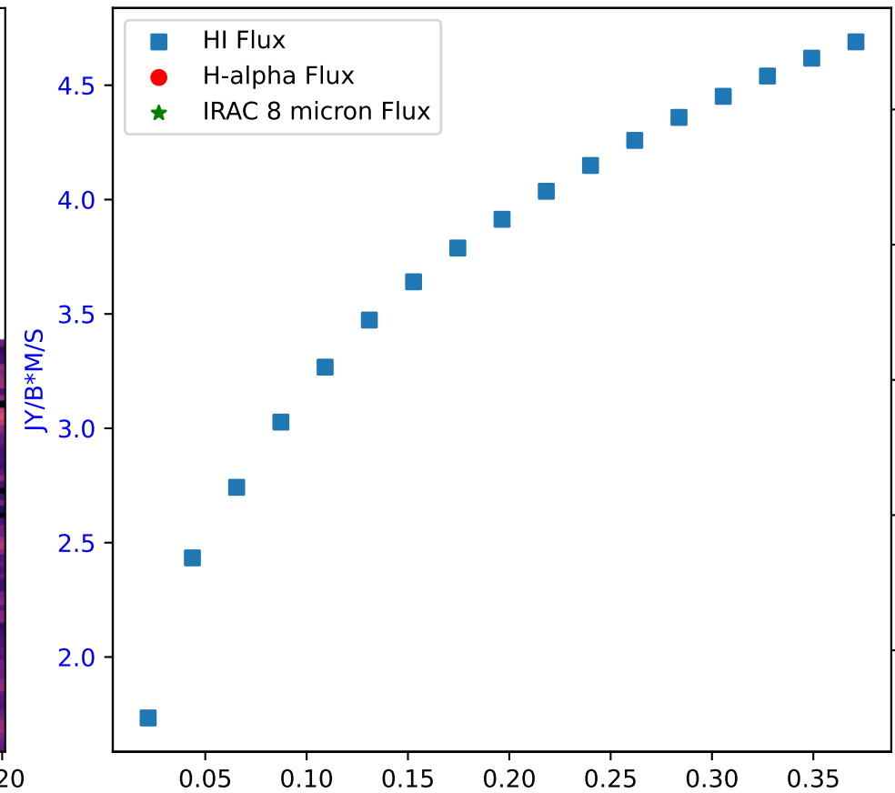
Flux of HI vs. H-alpha in Galaxy: NGC 4214 - Region 6
