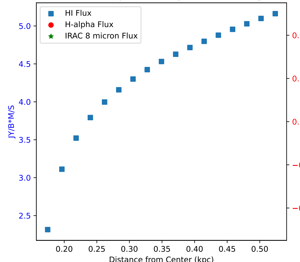
Flux of HI vs. H-alpha in Galaxy: NGC 4214 - Region 8
