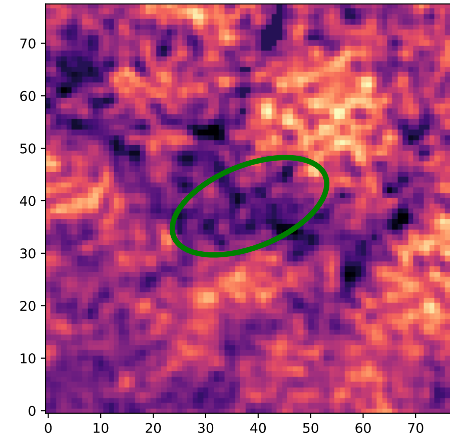
Region: 17 HI - Type 2
