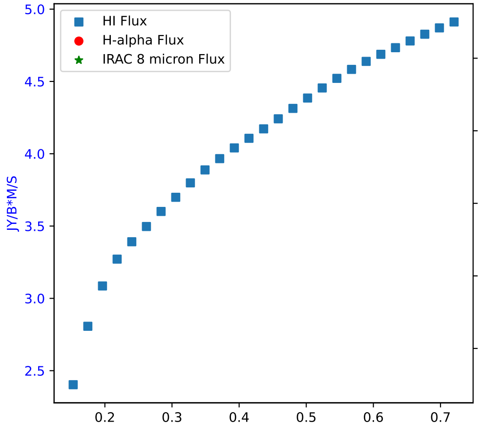
Flux of HI vs. H-alpha in Galaxy: NGC 4214 - Region 14
