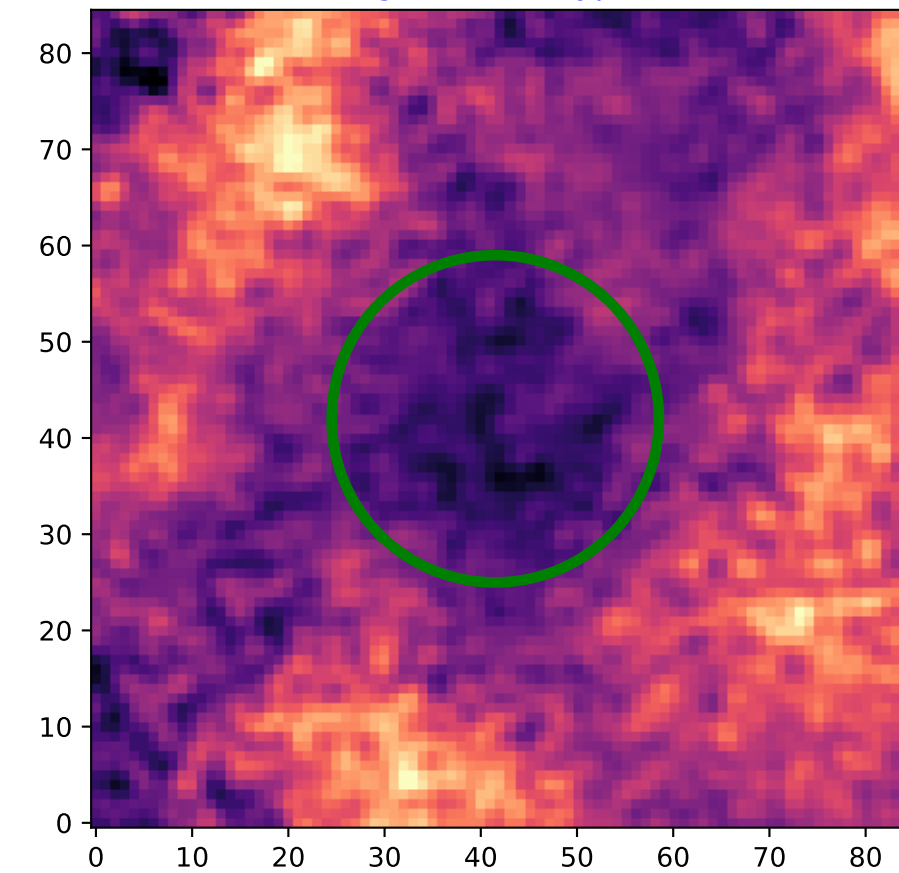
Region: 8 HI - Type 1
