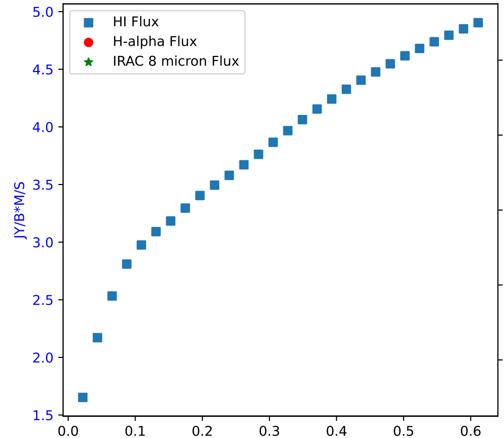
Flux of HI vs. H-alpha in Galaxy: NGC 4214 - Region 18
