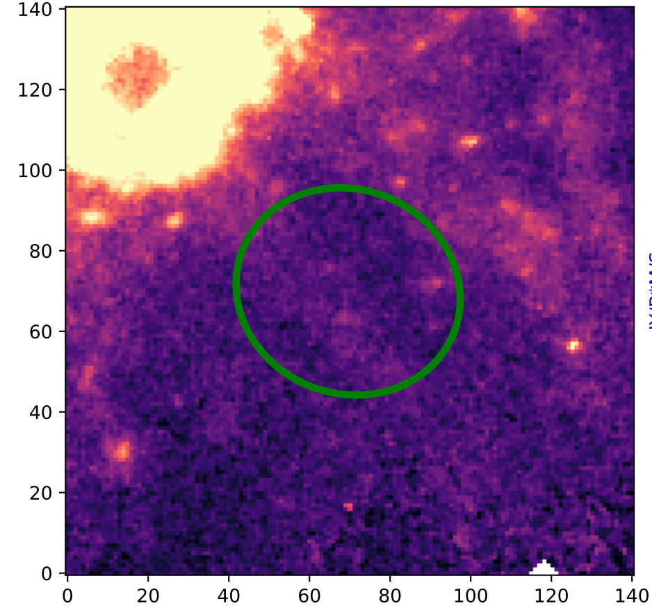
IRAC 8 micron - Classification: Diffuse
