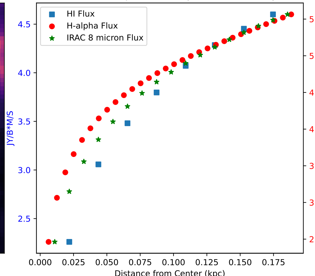
Flux of HI vs. H-alpha in Galaxy: NGC 4214 - Region 9
