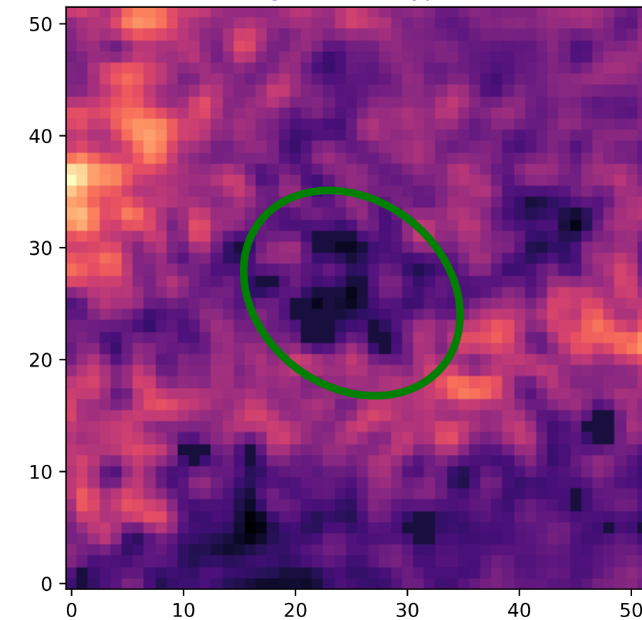
Region: 4 HI - Type 2
