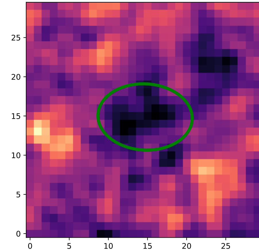
Region: 16 HI - Type 1
