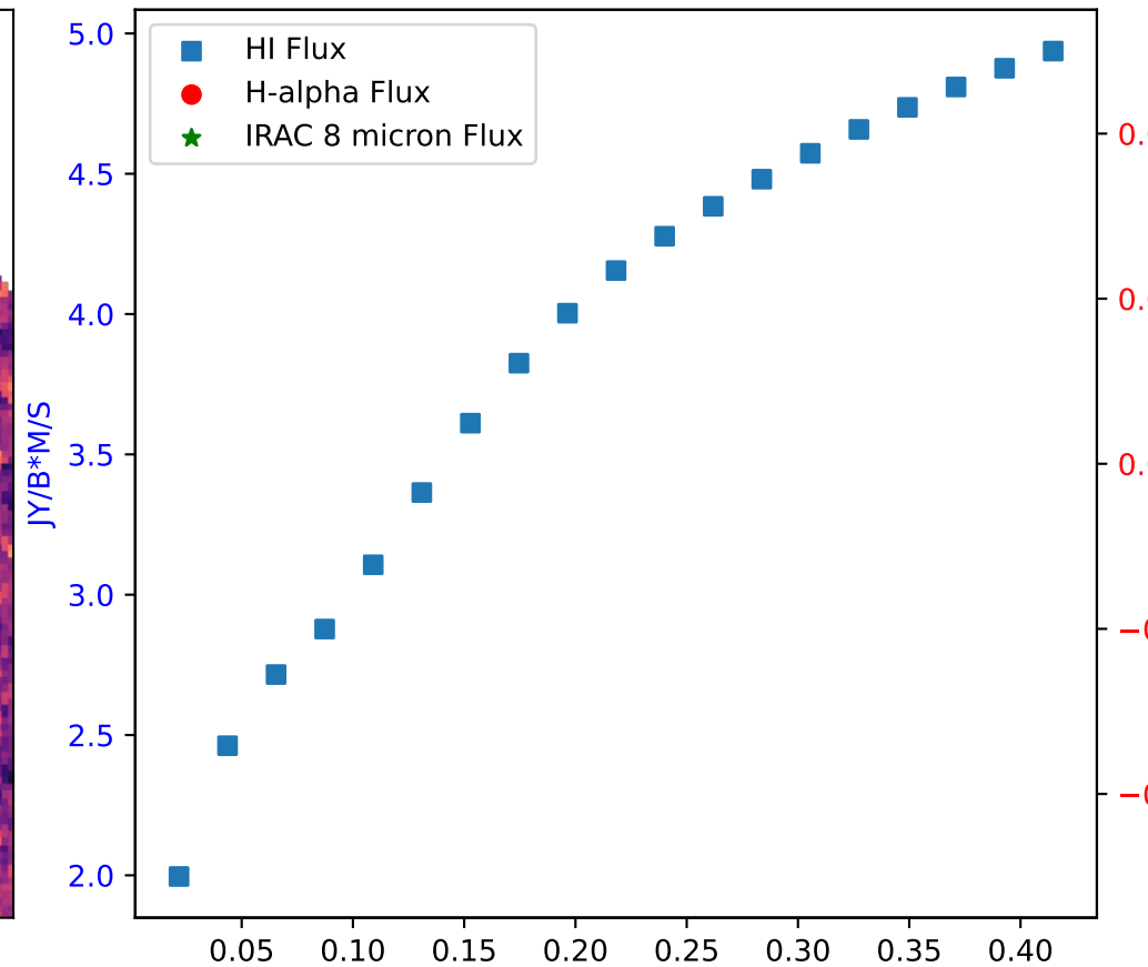
Flux of HI vs. H-alpha in Galaxy: NGC 4214 - Region 1
