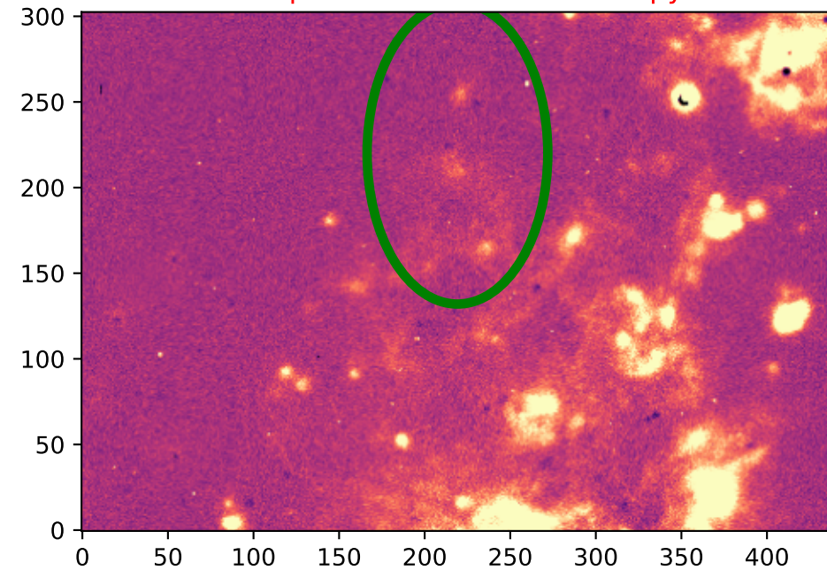
H-alpha - Classification: Clumpy
