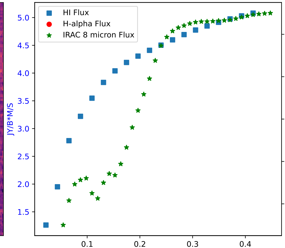
Flux of HI vs. H-alpha in Galaxy: NGC 4214 - Region 19
