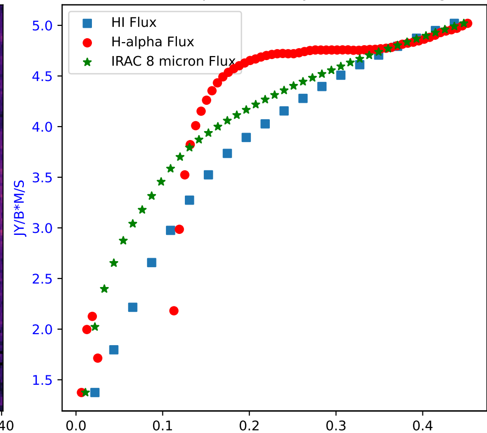
Flux of HI vs. H-alpha in Galaxy: NGC 4214 - Region 7
