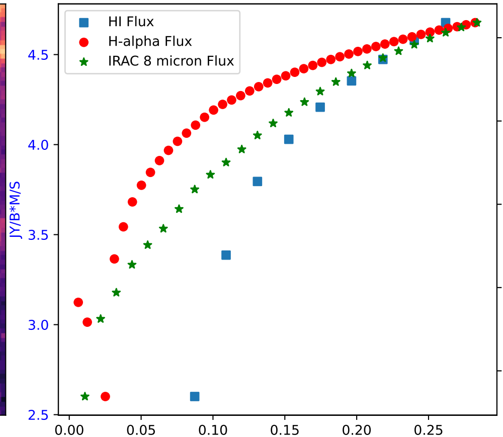
Flux of HI vs. H-alpha in Galaxy: NGC 4214 - Region 12
