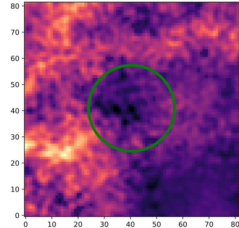
Region: 5 HI - Type 1
