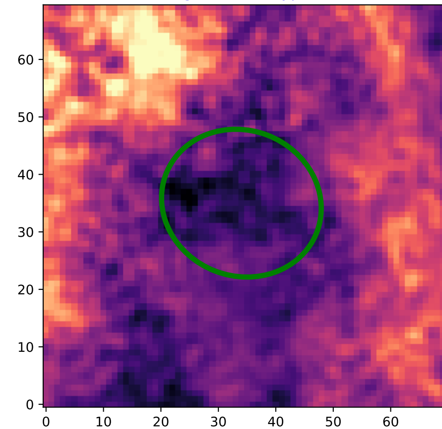
Region: 7 HI - Type 1
