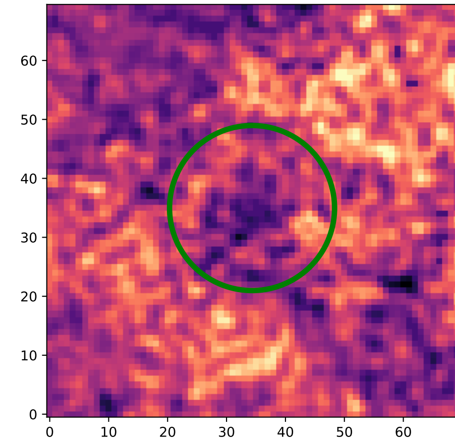
Region: 19 HI - Type 1
