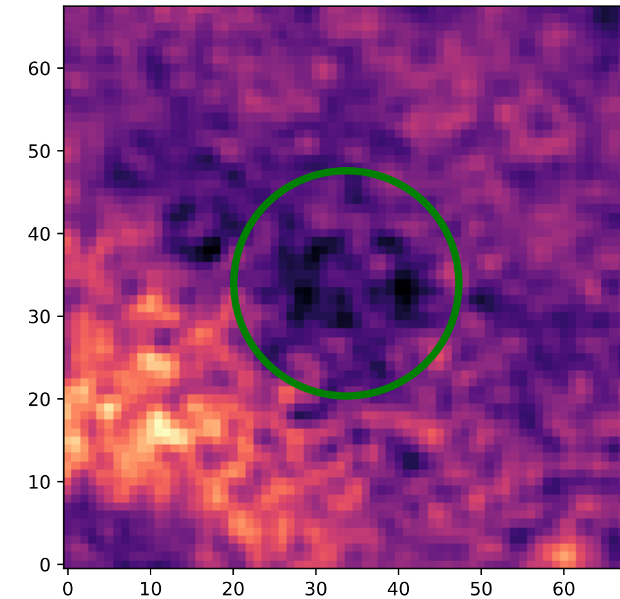
Region: 1 HI - Type 3
