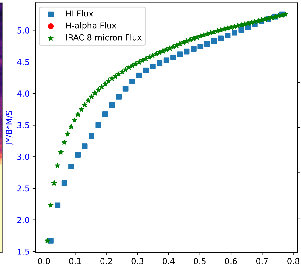
Flux of HI vs. H-alpha in Galaxy: NGC 4214 - Region 15
